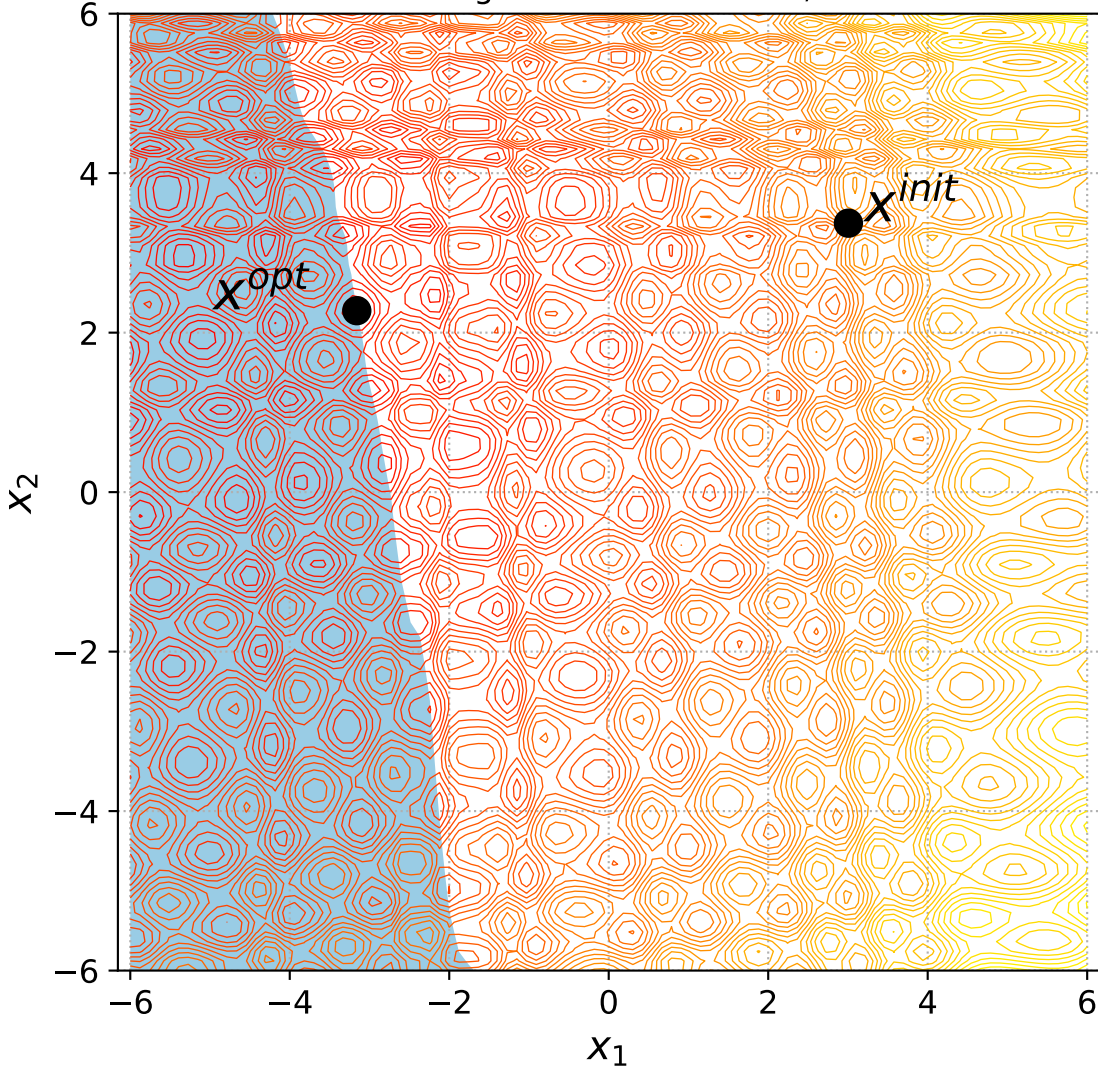
49 Rotated Rastrigin with 1 constraint, instance=15
