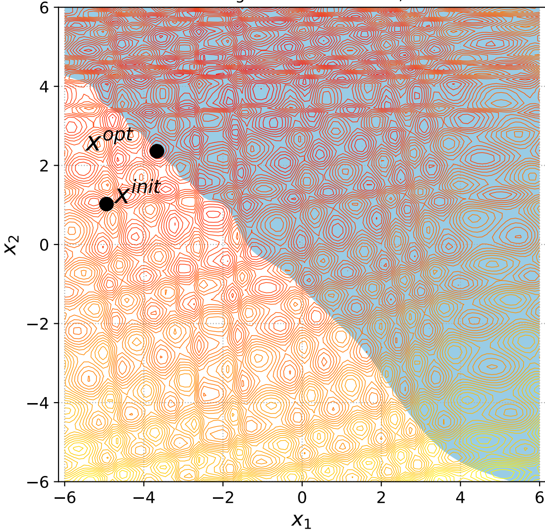
49 Rotated Rastrigin with 1 constraint, instance=14
