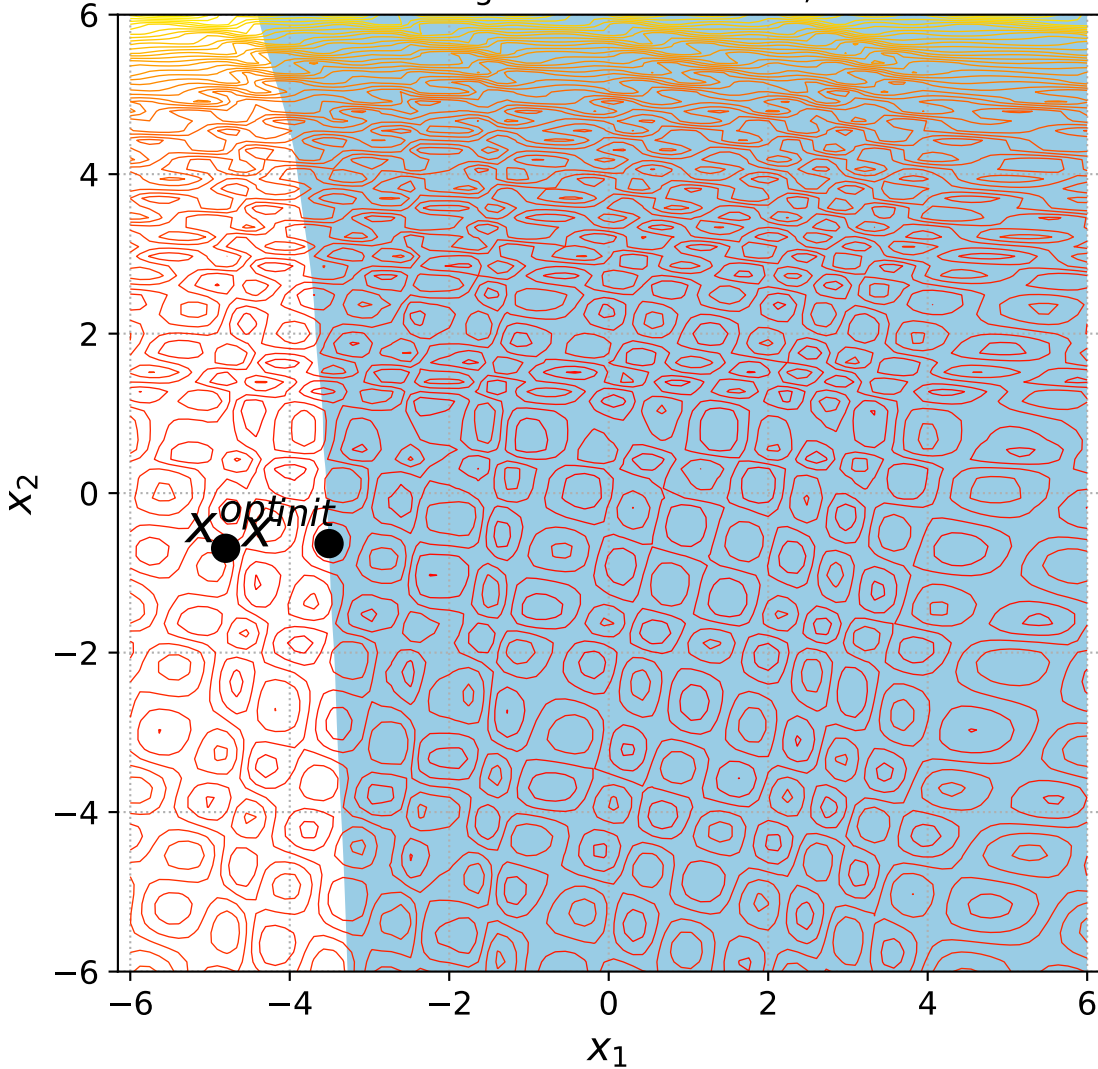
49 Rotated Rastrigin with 1 constraint, instance=13
