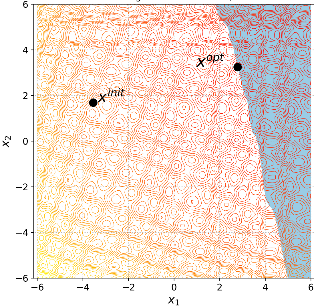
49 Rotated Rastrigin with 1 constraint, instance=11
