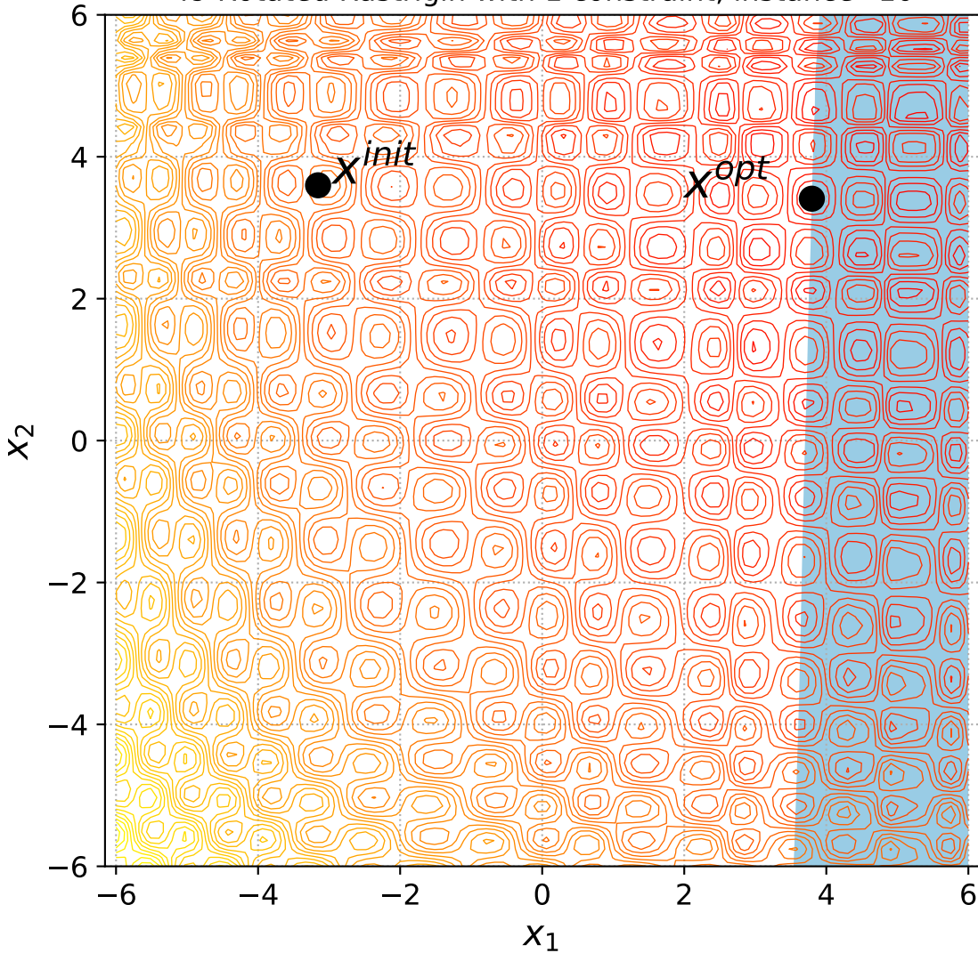
49 Rotated Rastrigin with 1 constraint, instance=10
