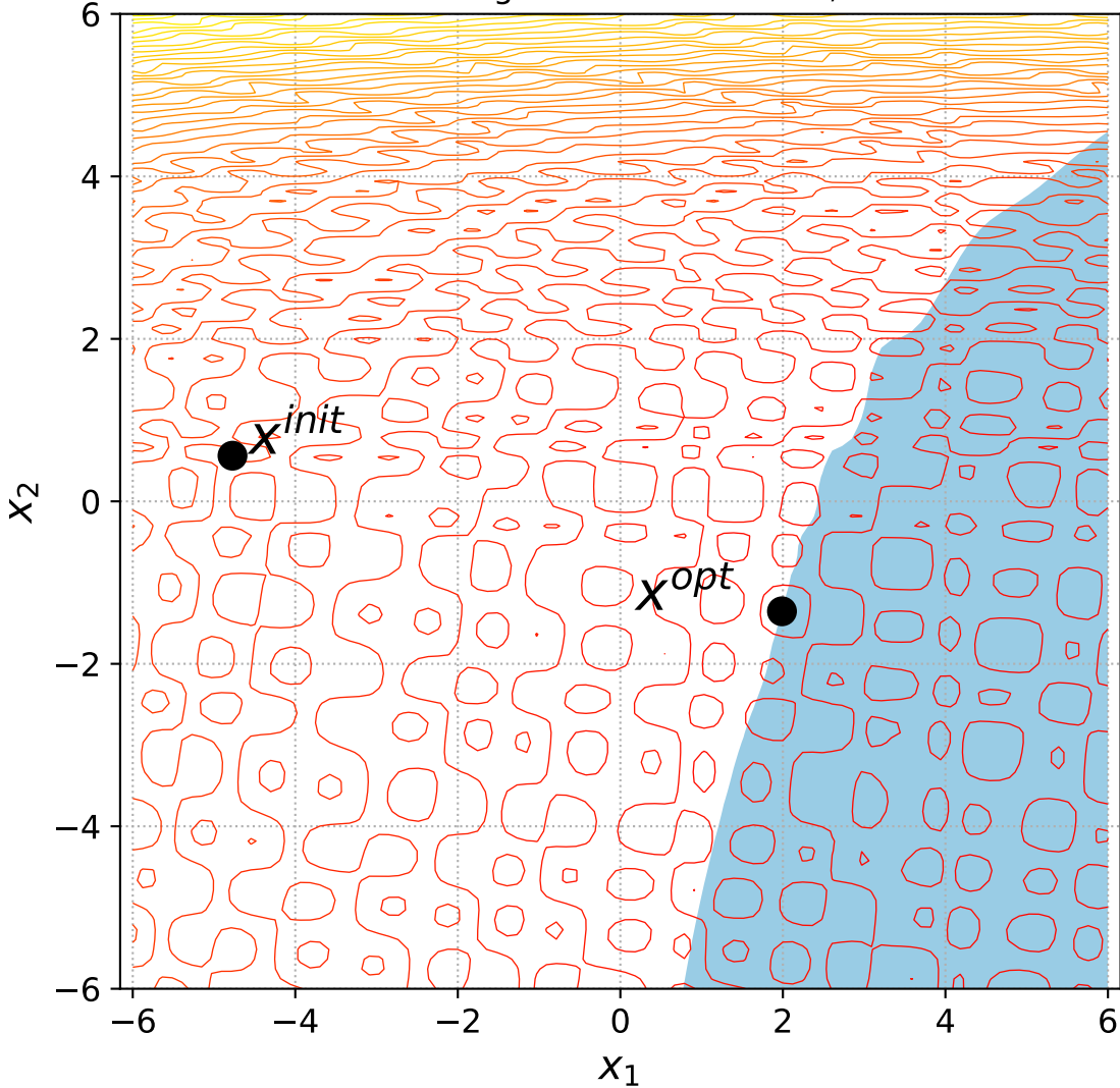
49 Rotated Rastrigin with 1 constraint, instance=9
