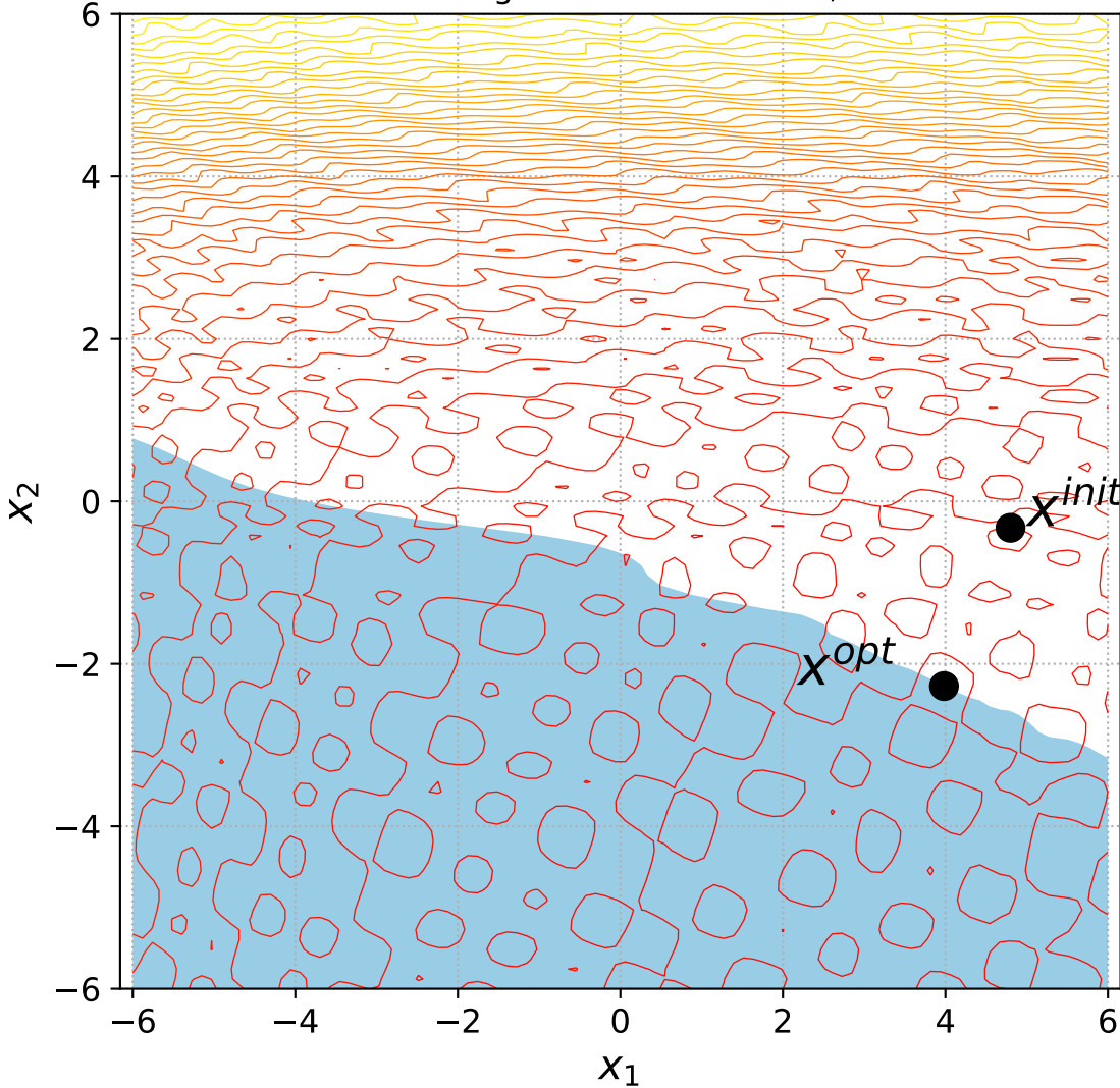
49 Rotated Rastrigin with 1 constraint, instance=8
