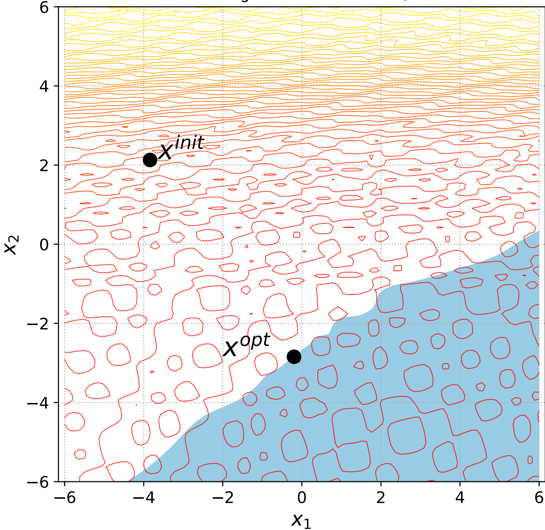
49 Rotated Rastrigin with 1 constraint, instance=7
