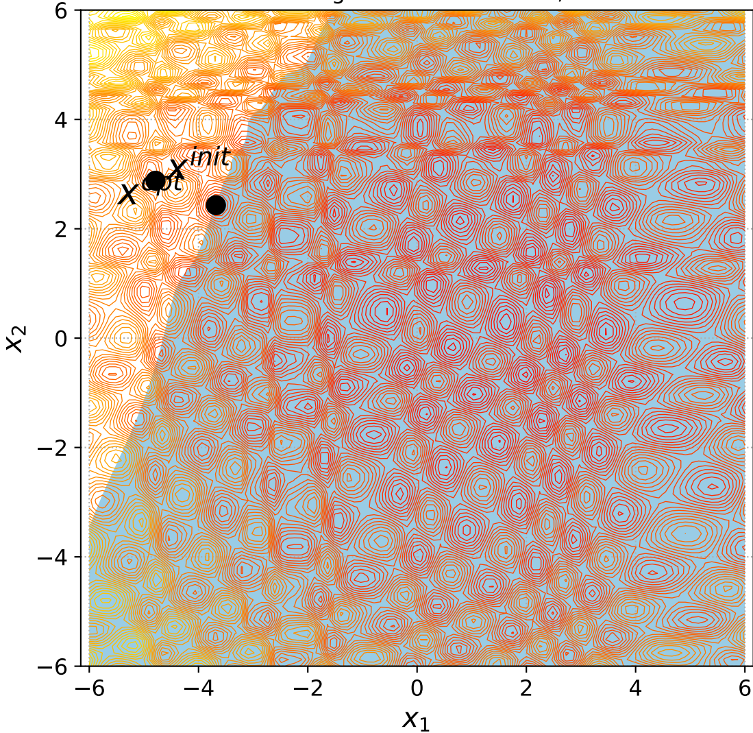
49 Rotated Rastrigin with 1 constraint, instance=6
