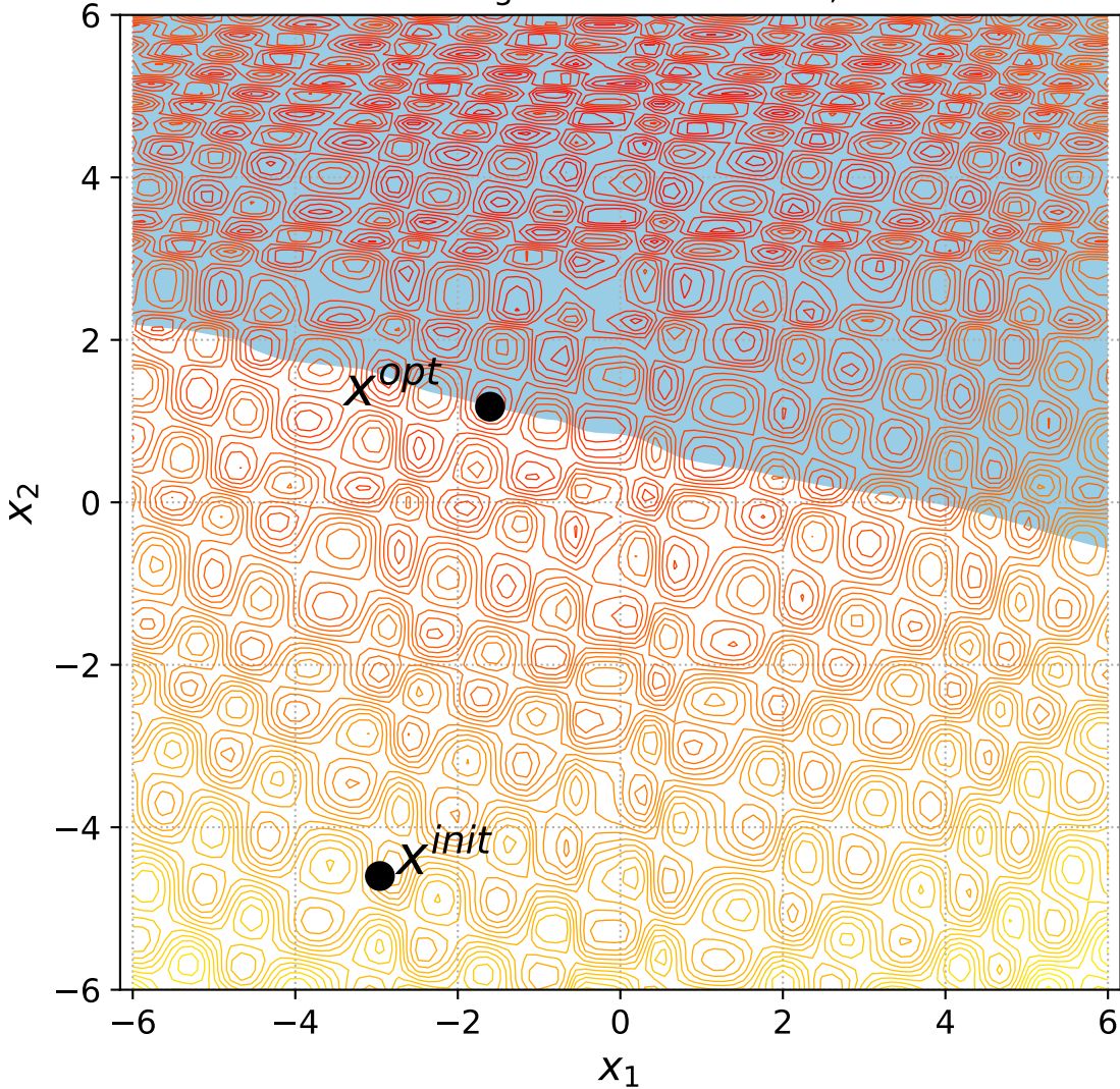
49 Rotated Rastrigin with 1 constraint, instance=5
