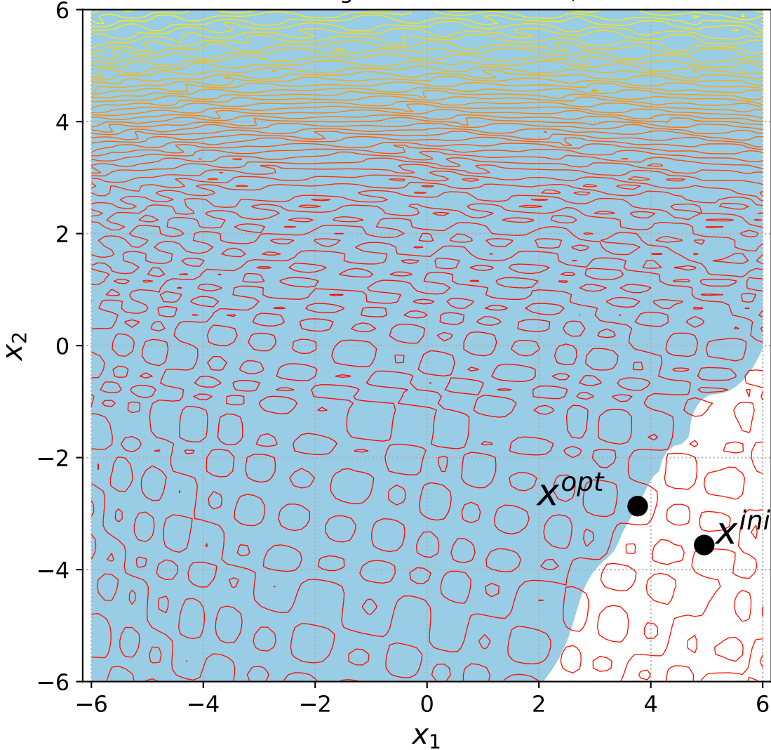
49 Rotated Rastrigin with 1 constraint, instance=4
