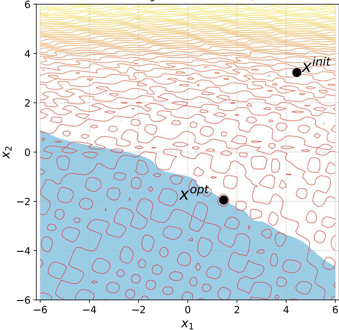
49 Rotated Rastrigin with 1 constraint, instance=3
