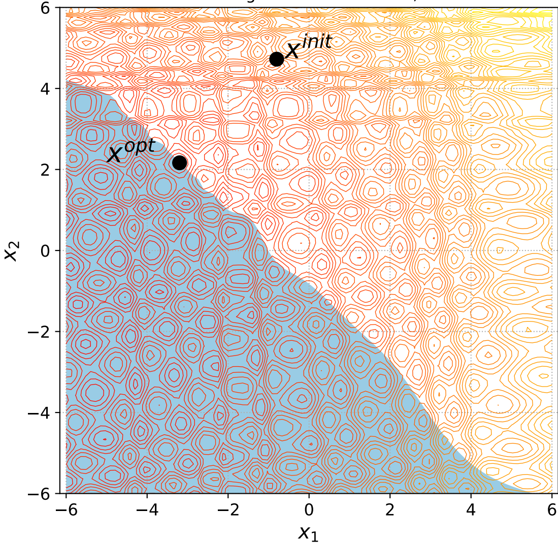
49 Rotated Rastrigin with 1 constraint, instance=2
