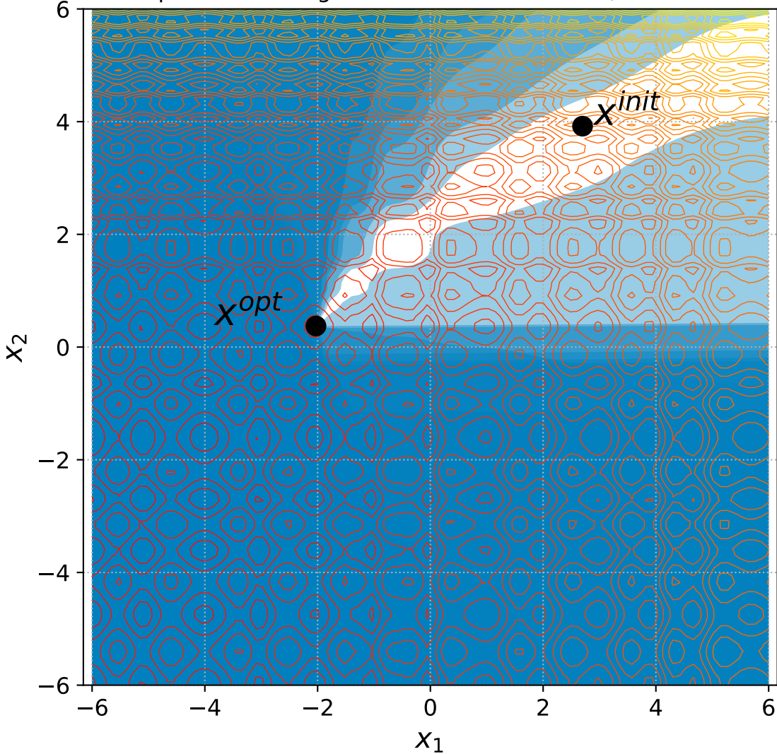
48 Separable Rastrigin with 6+3n constraints, instance=15
