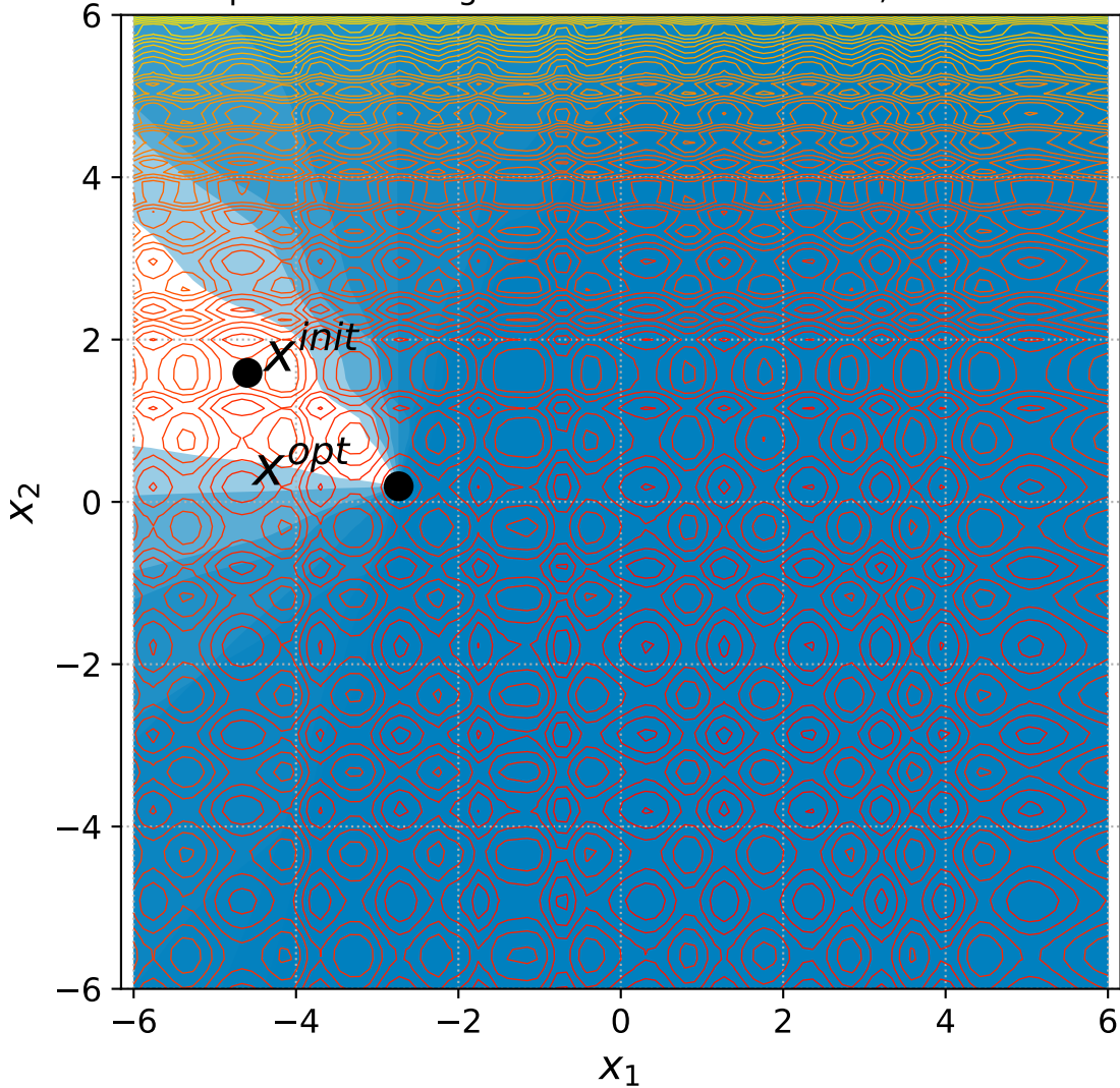
48 Separable Rastrigin with 6+3n constraints, instance=12
