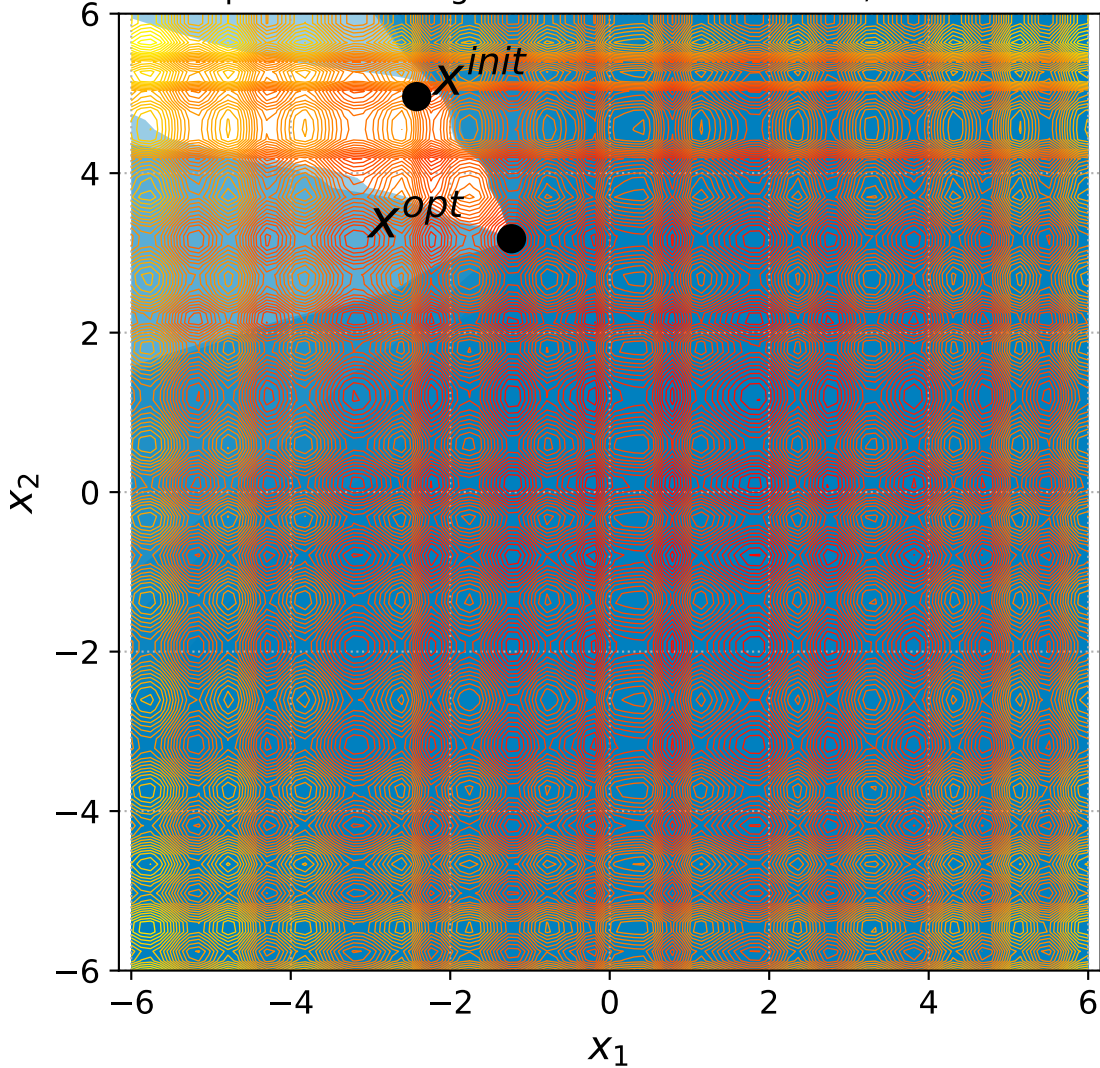
48 Separable Rastrigin with 6+3n constraints, instance=11
