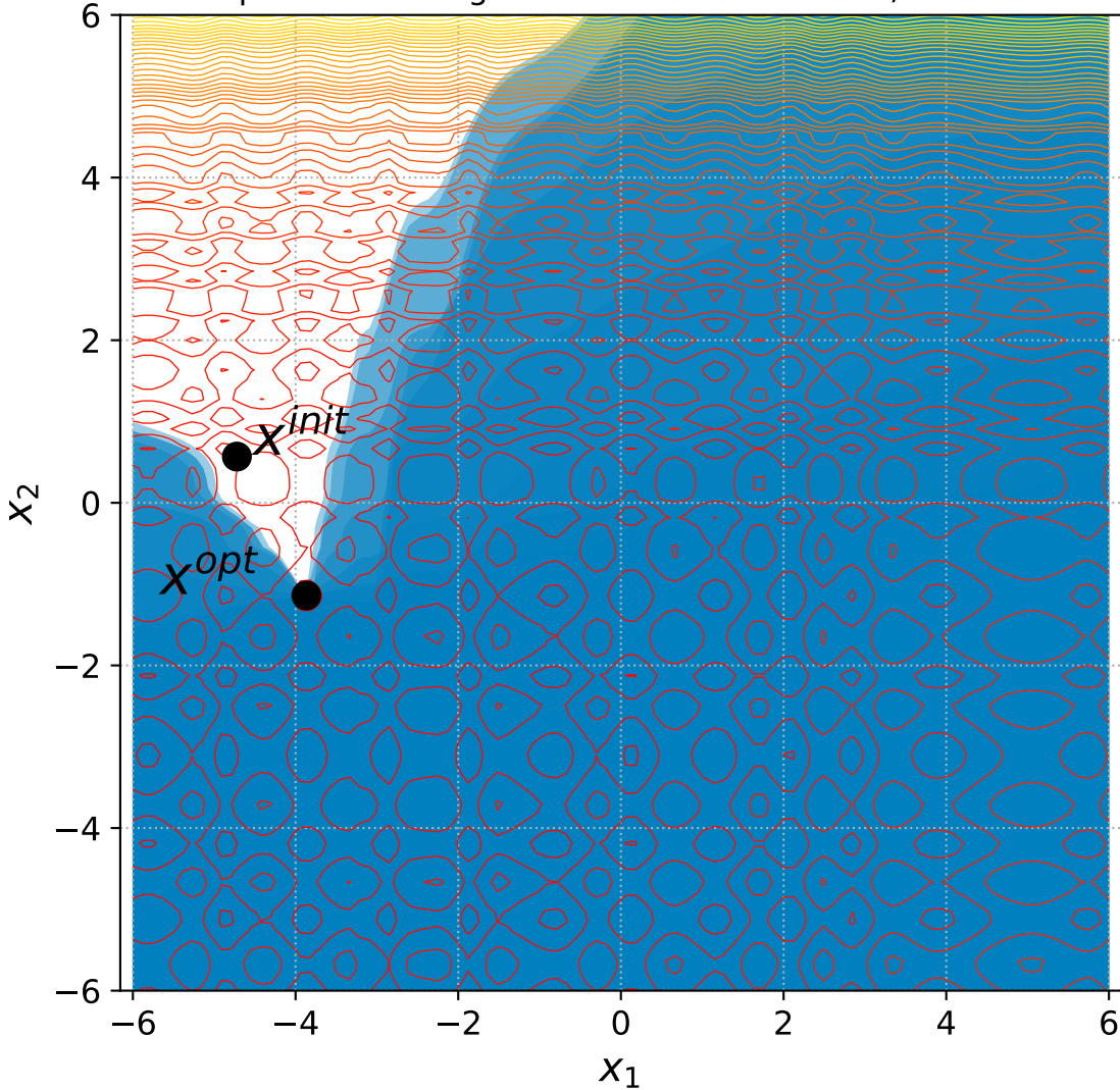
48 Separable Rastrigin with 6+3n constraints, instance=9
