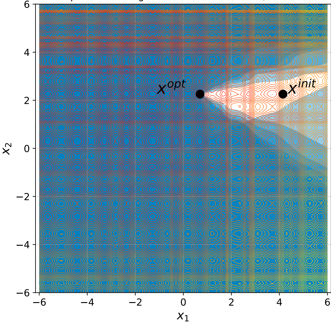
48 Separable Rastrigin with 6+3n constraints, instance=8
