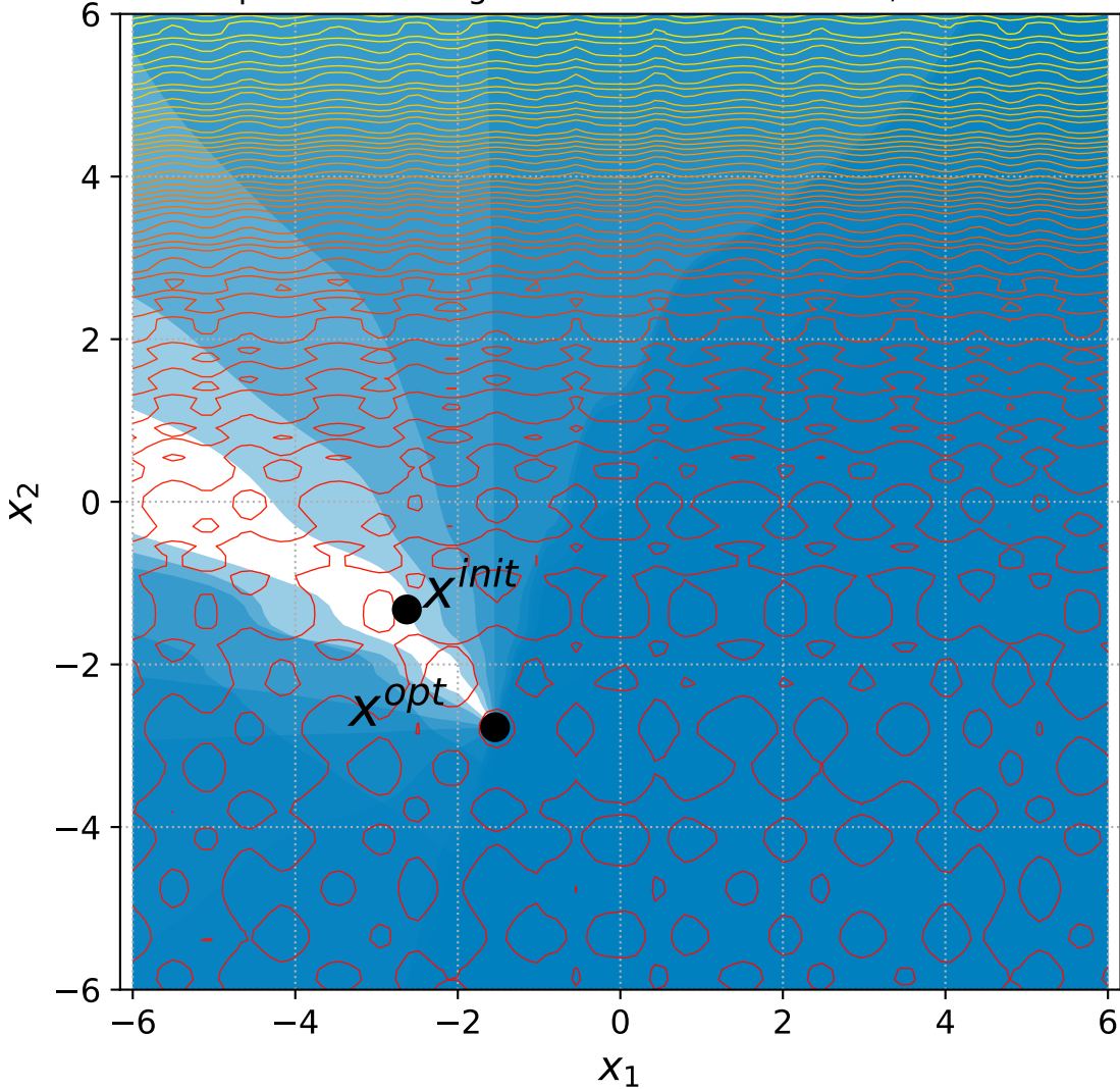
48 Separable Rastrigin with 6+3n constraints, instance=7
