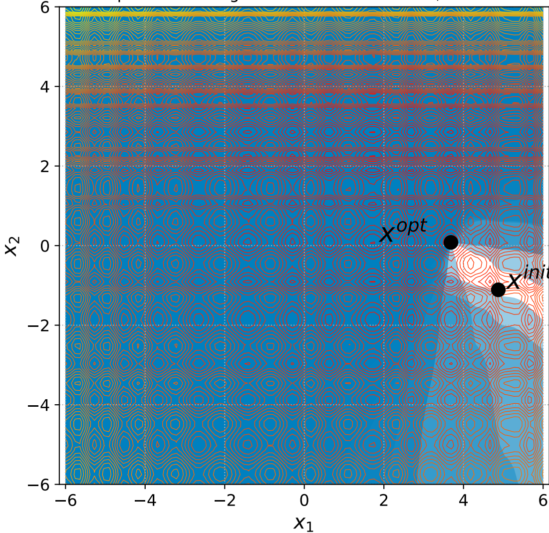
48 Separable Rastrigin with 6+3n constraints, instance=5
