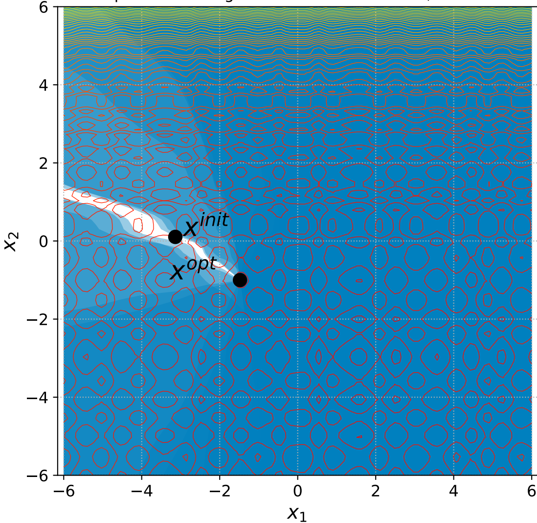
48 Separable Rastrigin with 6+3n constraints, instance=3
