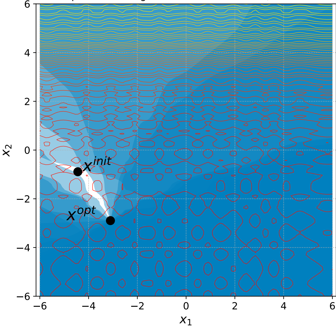
48 Separable Rastrigin with 6+3n constraints, instance=2
