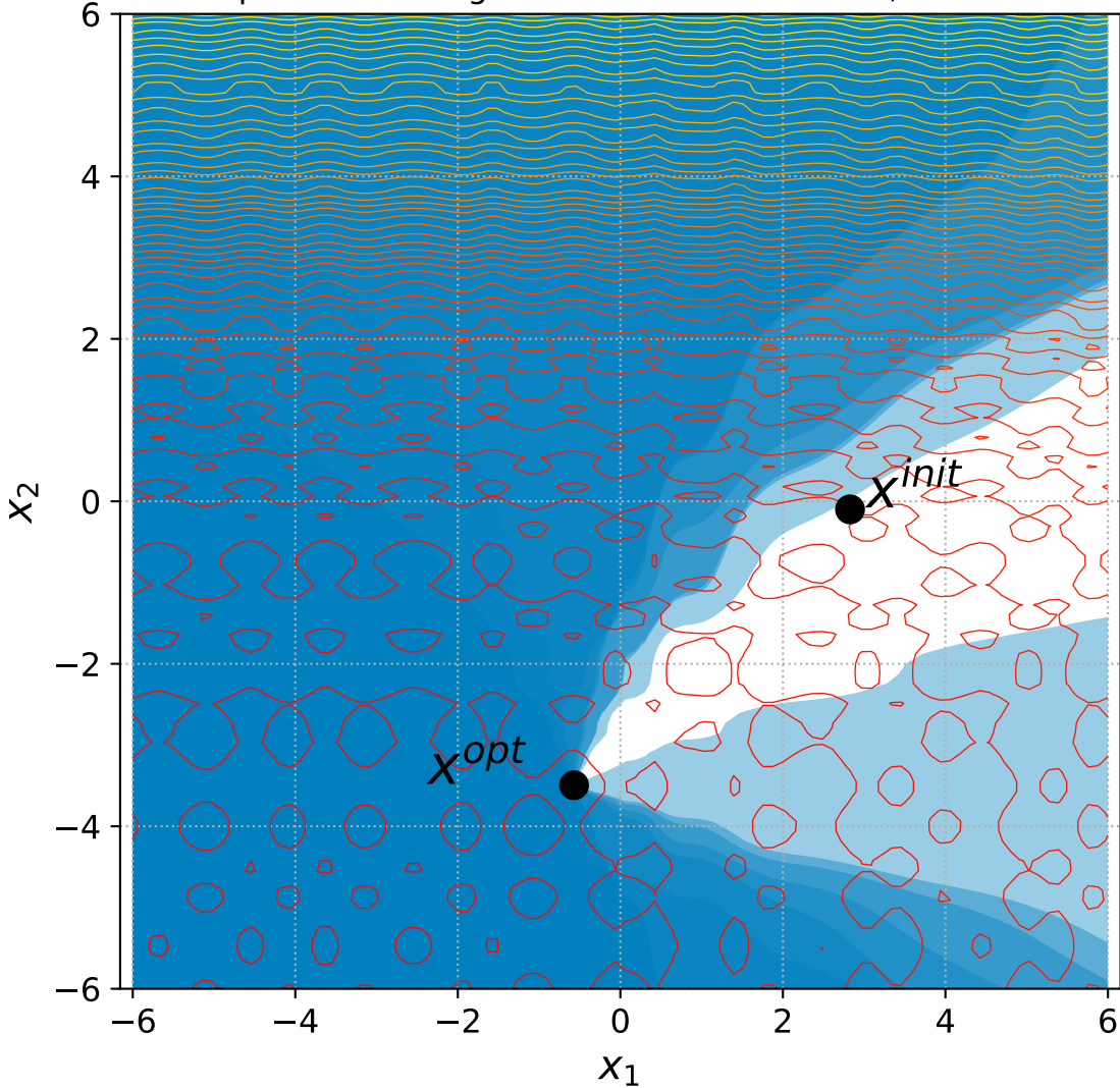
48 Separable Rastrigin with 6+3n constraints, instance=1
