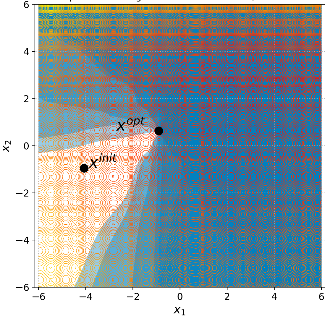
47 Separable Rastrigin with 6+n constraints, instance=15
