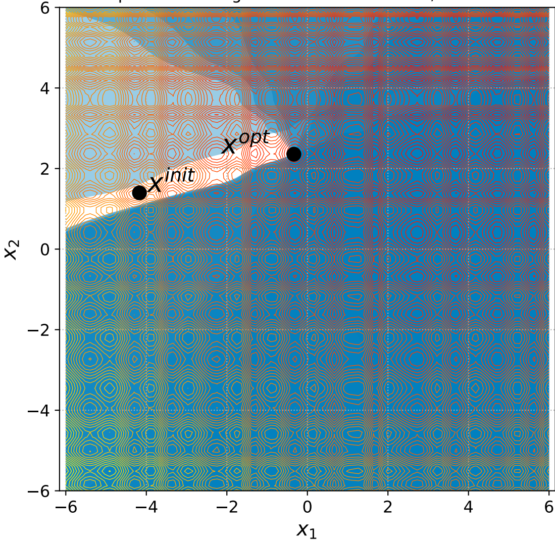
47 Separable Rastrigin with 6+n constraints, instance=14
