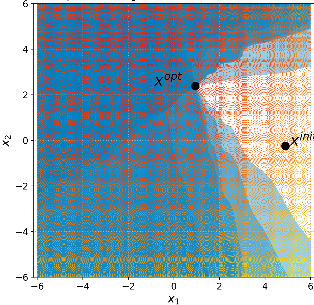
47 Separable Rastrigin with 6+n constraints, instance=13
