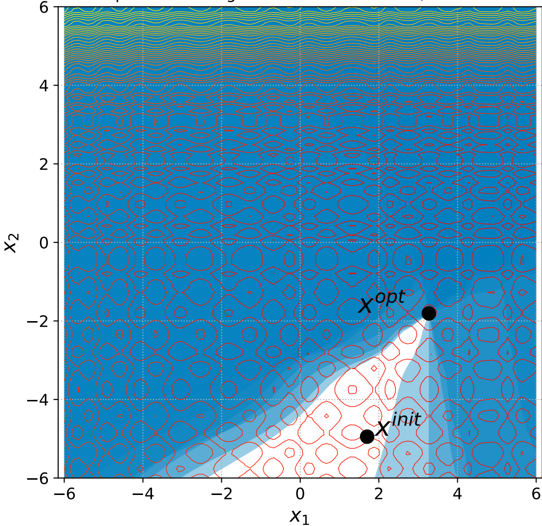
47 Separable Rastrigin with 6+n constraints, instance=12
