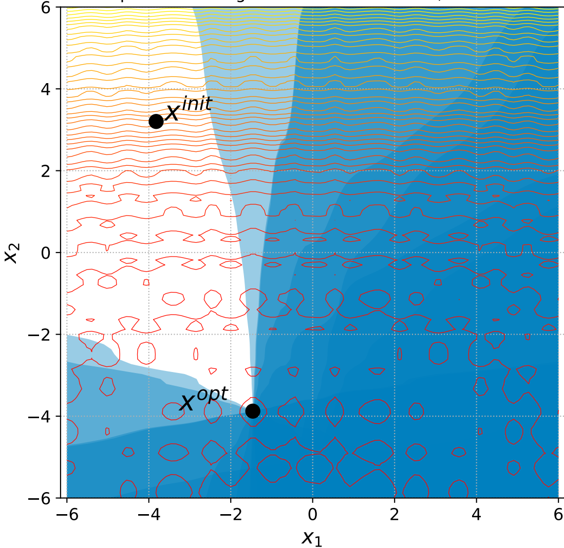
47 Separable Rastrigin with 6+n constraints, instance=10
