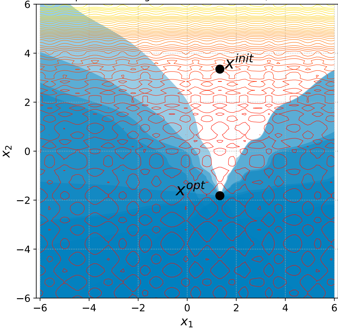
47 Separable Rastrigin with 6+n constraints, instance=8
