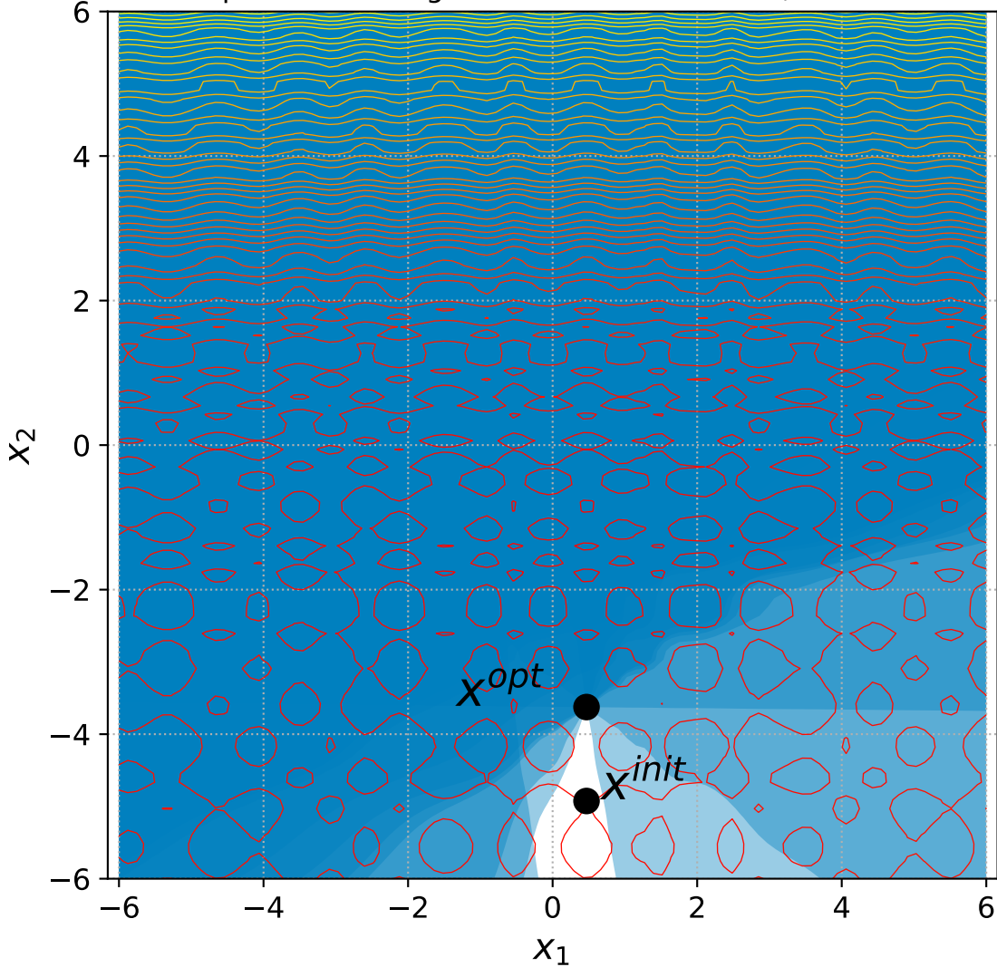
47 Separable Rastrigin with 6+n constraints, instance=7
