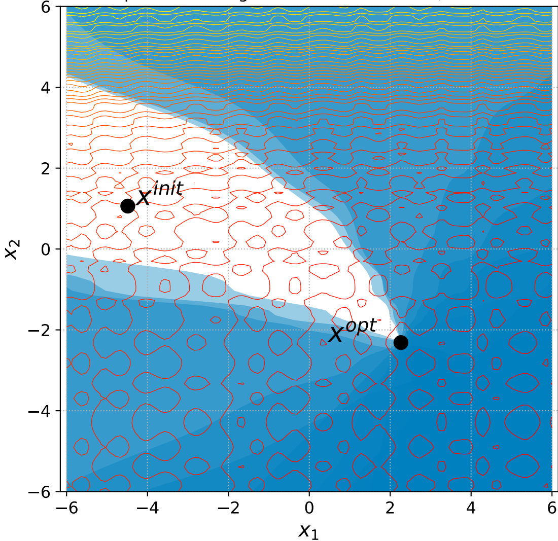
47 Separable Rastrigin with 6+n constraints, instance=6
