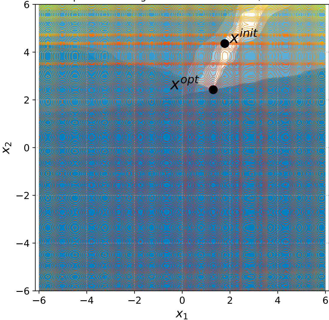
47 Separable Rastrigin with 6+n constraints, instance=5
