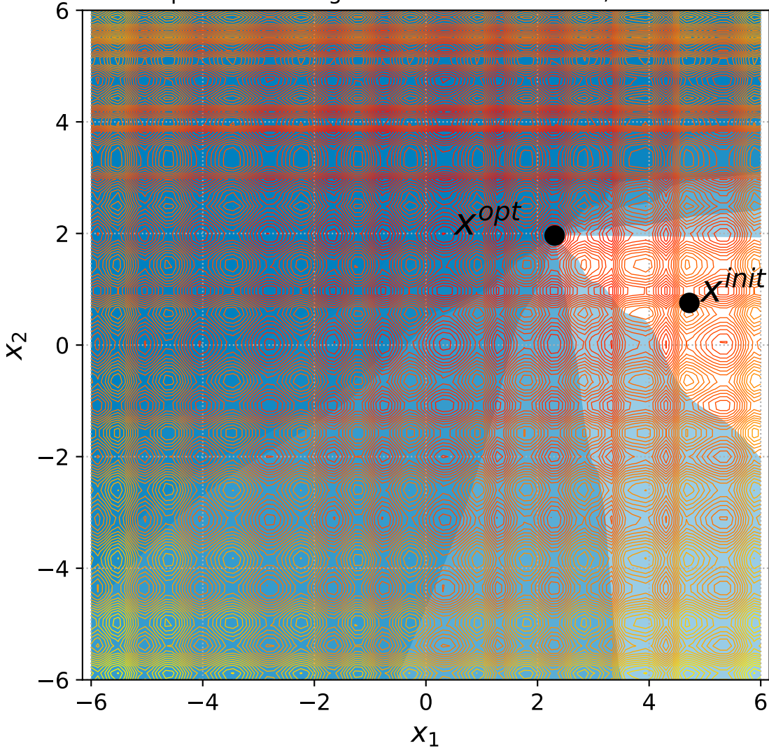
47 Separable Rastrigin with 6+n constraints, instance=2
