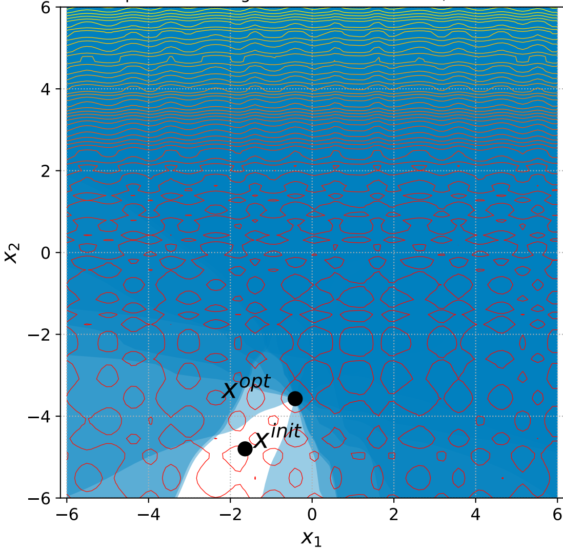
47 Separable Rastrigin with 6+n constraints, instance=1
