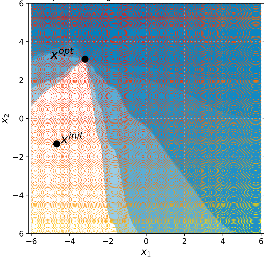
46 Separable Rastrigin with 6+n/2 constraints, instance=15
