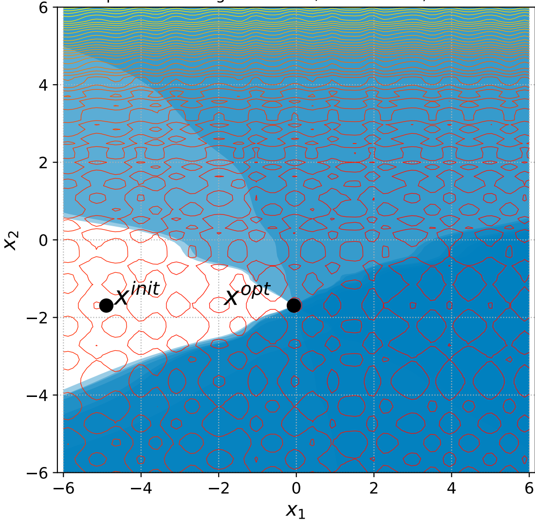
46 Separable Rastrigin with 6+n/2 constraints, instance=14
