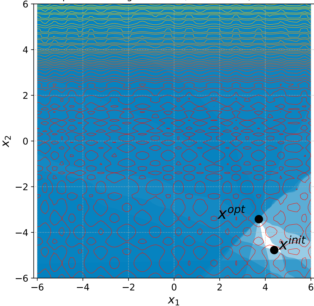
46 Separable Rastrigin with 6+n/2 constraints, instance=13
