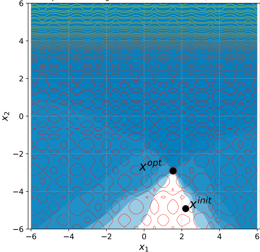
46 Separable Rastrigin with 6+n/2 constraints, instance=12
