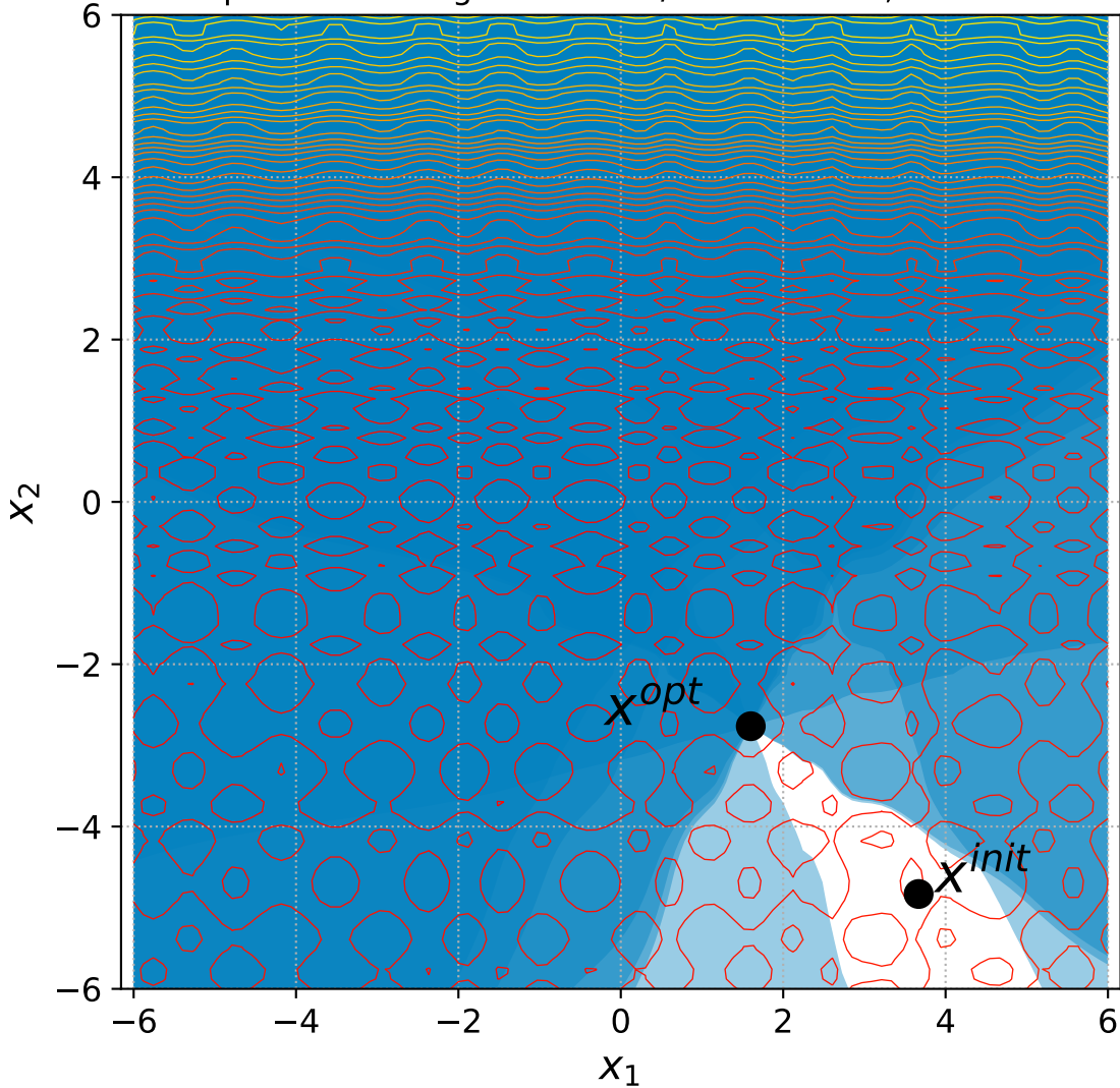
46 Separable Rastrigin with 6+n/2 constraints, instance=11
