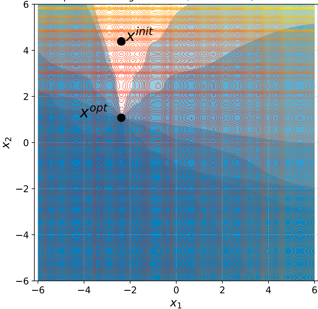
46 Separable Rastrigin with 6+n/2 constraints, instance=10
