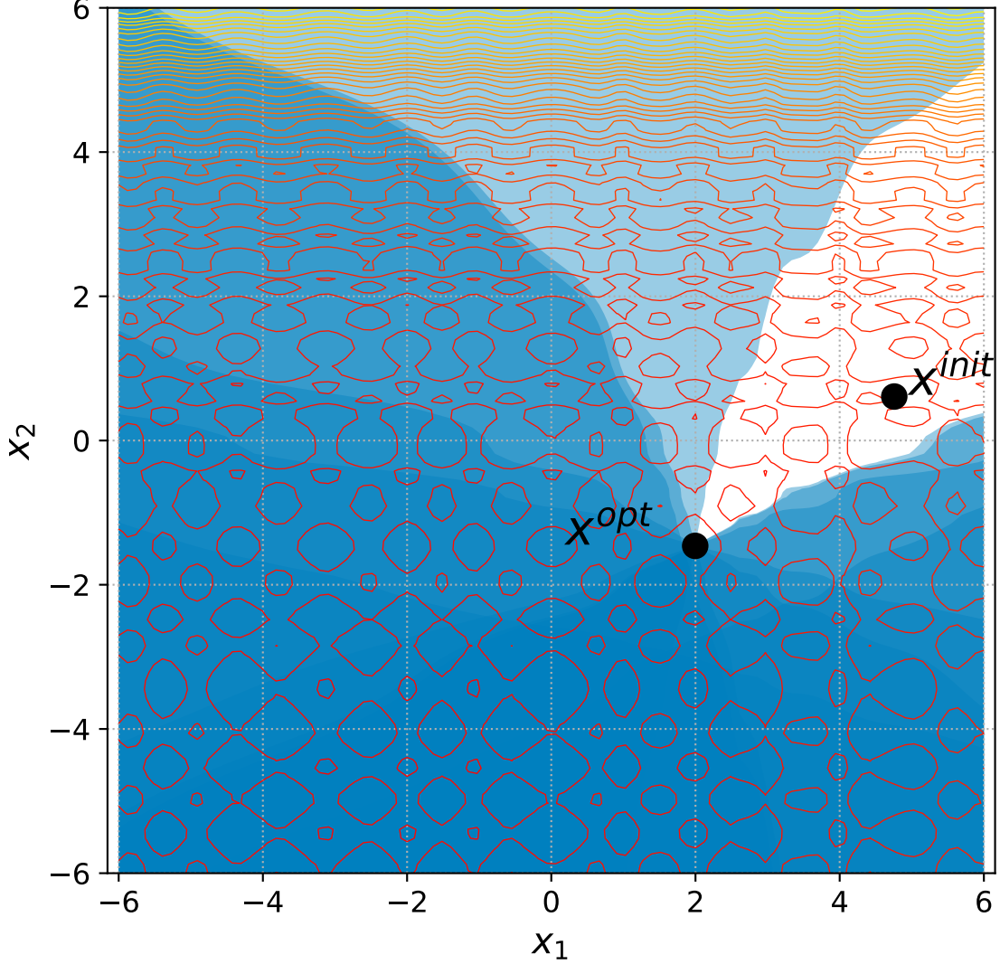
46 Separable Rastrigin with 6+n/2 constraints, instance=9
