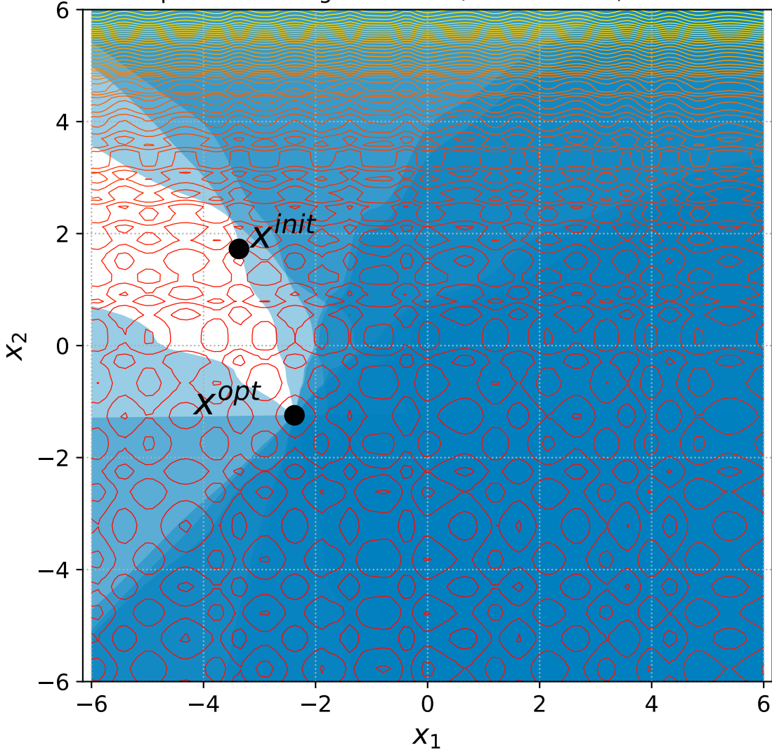
46 Separable Rastrigin with 6+n/2 constraints, instance=8
