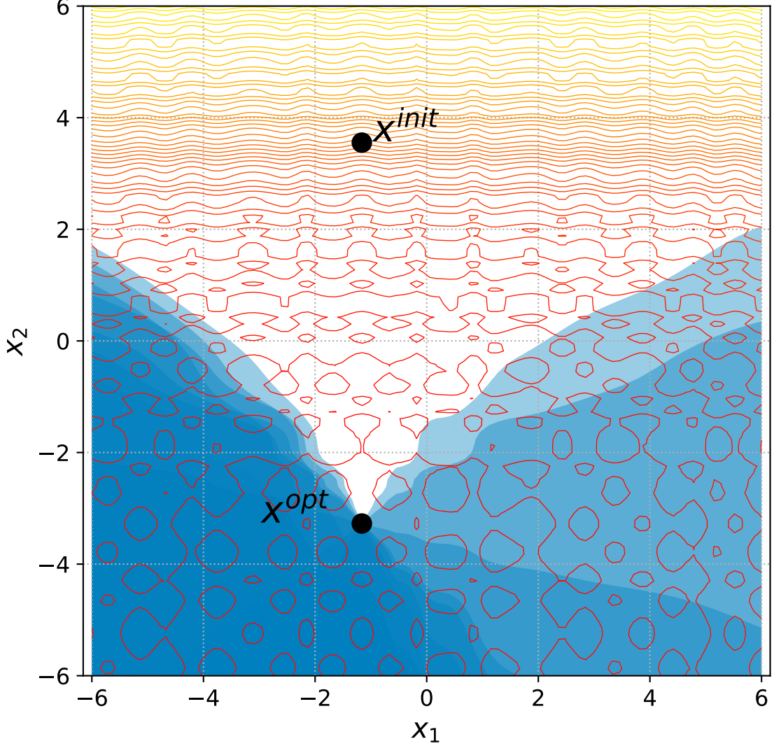
46 Separable Rastrigin with 6+n/2 constraints, instance=7
