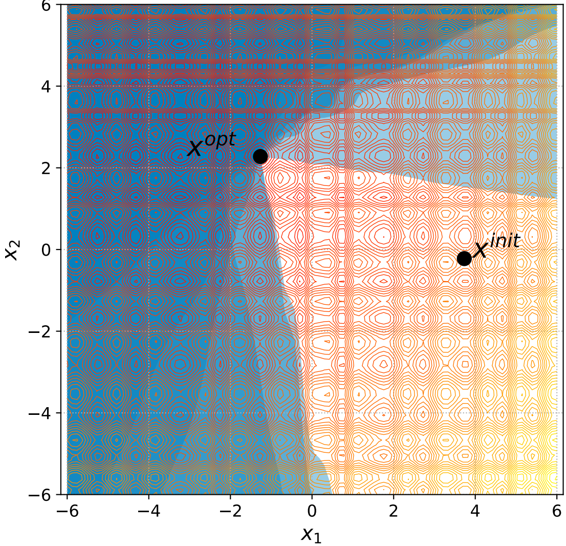
46 Separable Rastrigin with 6+n/2 constraints, instance=5
