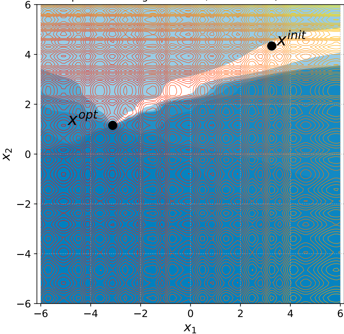
46 Separable Rastrigin with 6+n/2 constraints, instance=4
