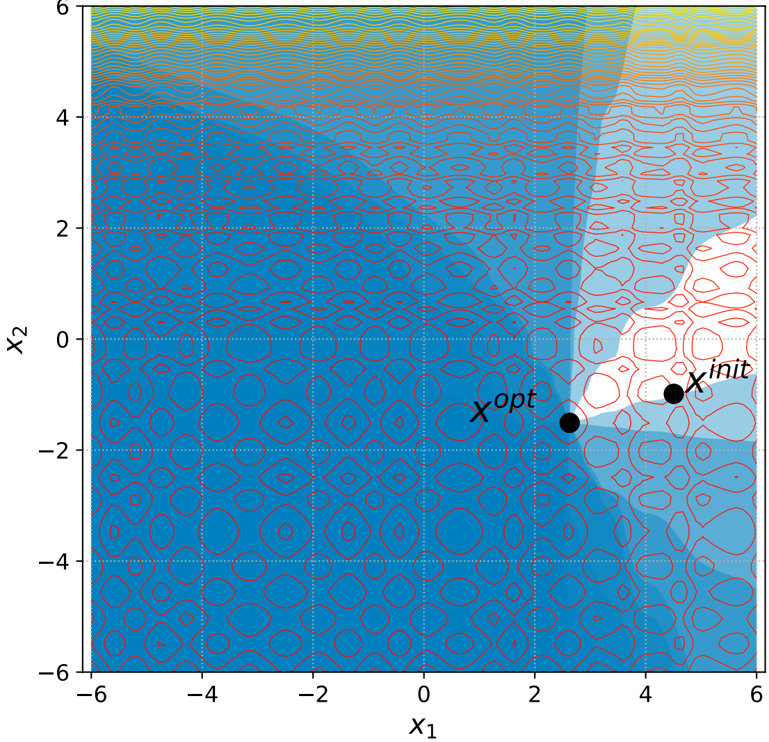
46 Separable Rastrigin with 6+n/2 constraints, instance=1
