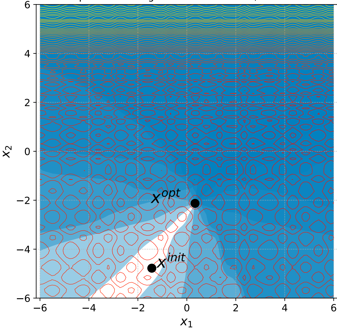
45 Separable Rastrigin with 6 constraints, instance=14
