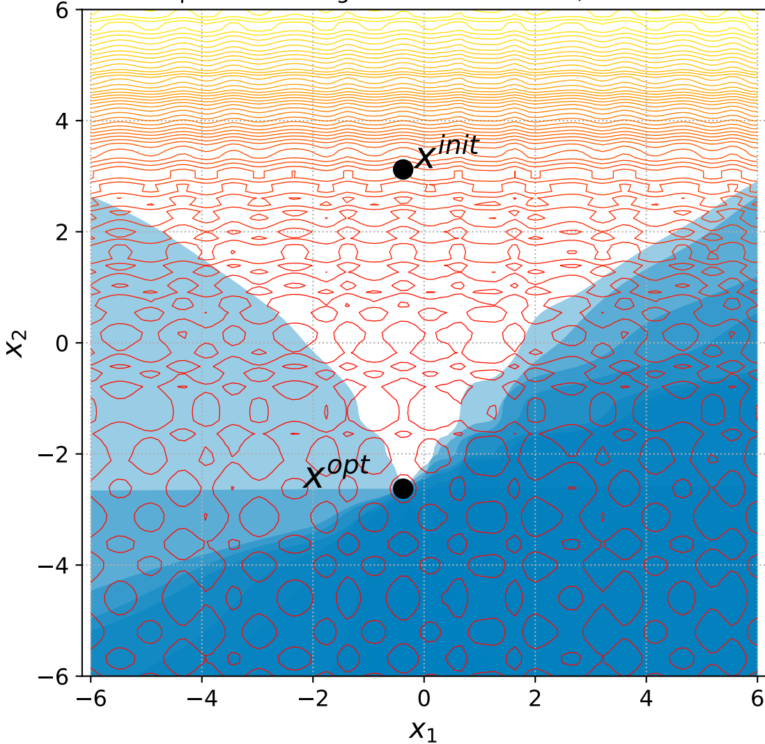
45 Separable Rastrigin with 6 constraints, instance=13
