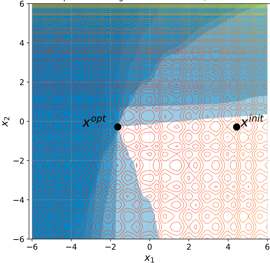
45 Separable Rastrigin with 6 constraints, instance=12
