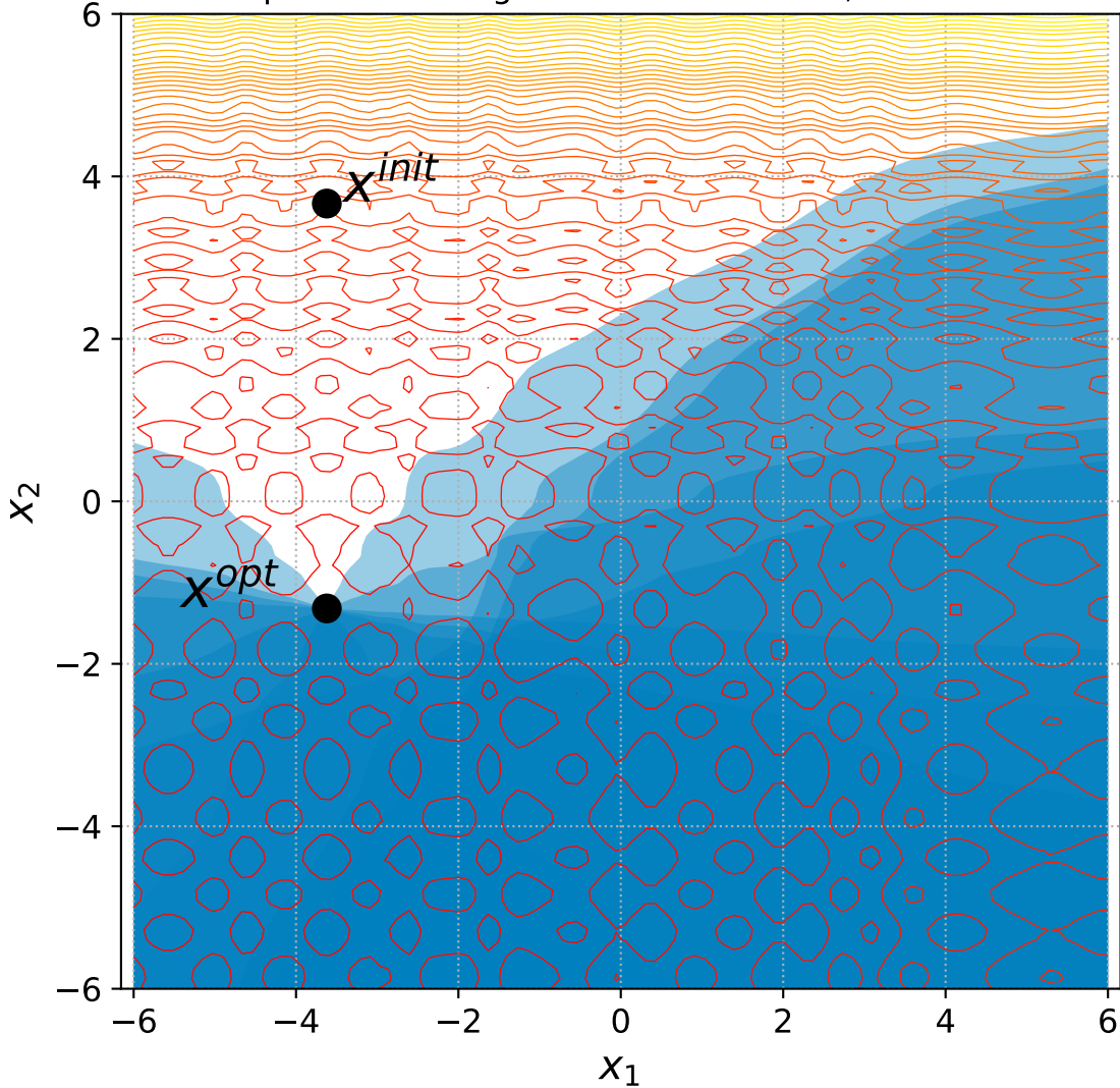
45 Separable Rastrigin with 6 constraints, instance=10
